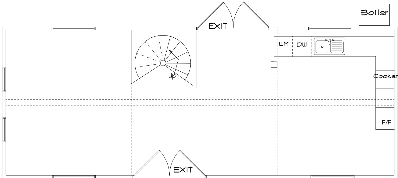
FIRST FLOOR Hop Barn
